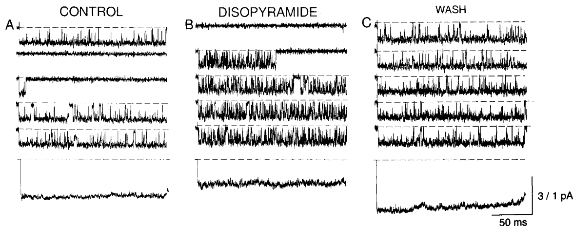
FIGURE 8 Effects of disopyramide on single sodium channel currents. Single sodium channel currents were recorded from a cell-attached membrane patch during control ( A ), exposure to disopyramide ( B ), and after washout of the drug ( C ). The holding potential was -90 mV and the test potential -20 mV. Each panel shows membrane current during five consecutive trials and the average current of 100 trials. There was evidence for a single functioning channel in this patch.
